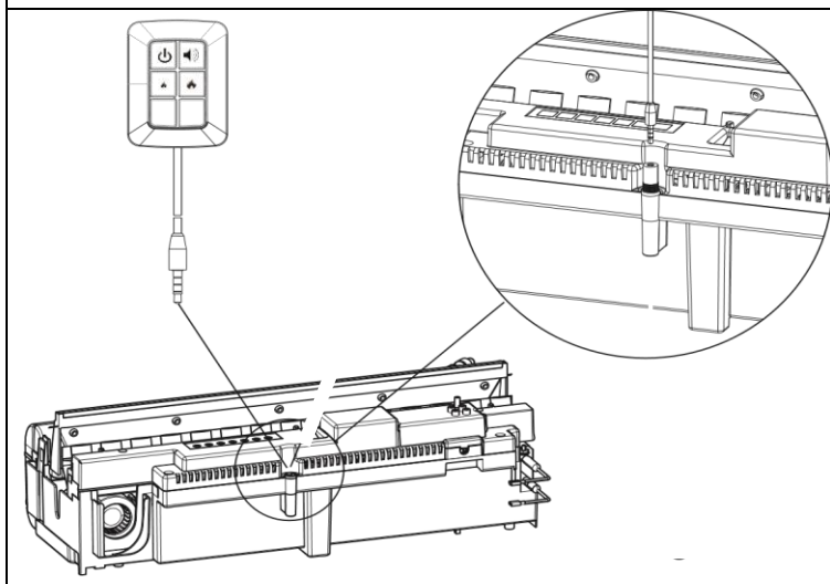
Fig 5 Setting the controller
