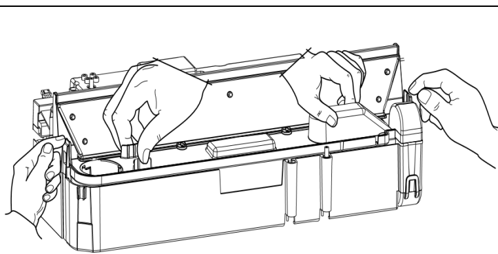
Fig 12 Sump locks
