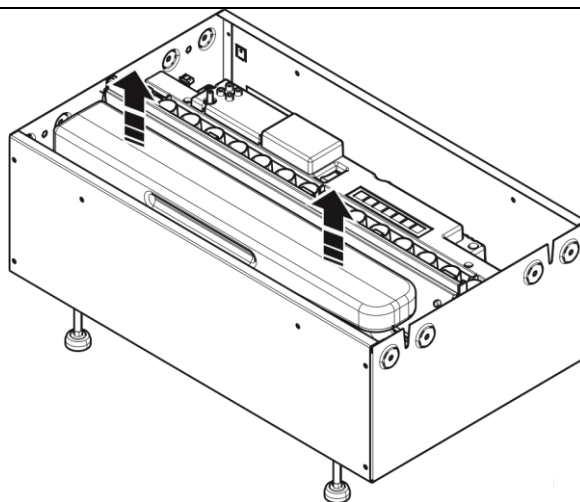
Fig 6 Lifting up the water tank
