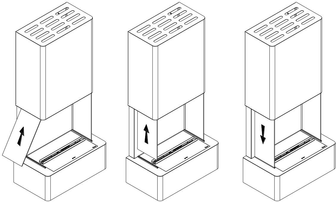
Fig 2 Glass installation
