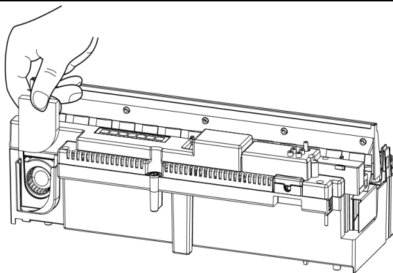
Fig 15 Air filter
